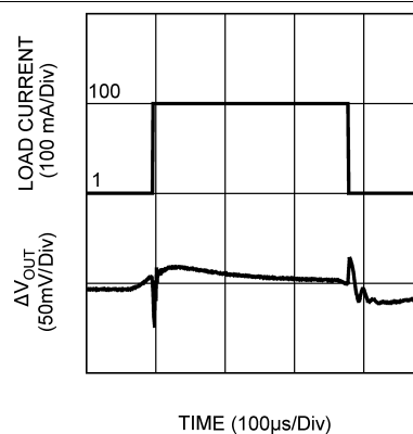
Figure 10. Load Transient
