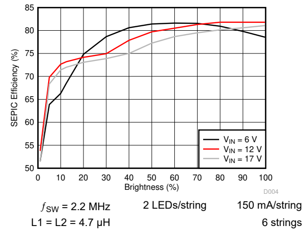
图 6-5. SEPIC Efficiency
