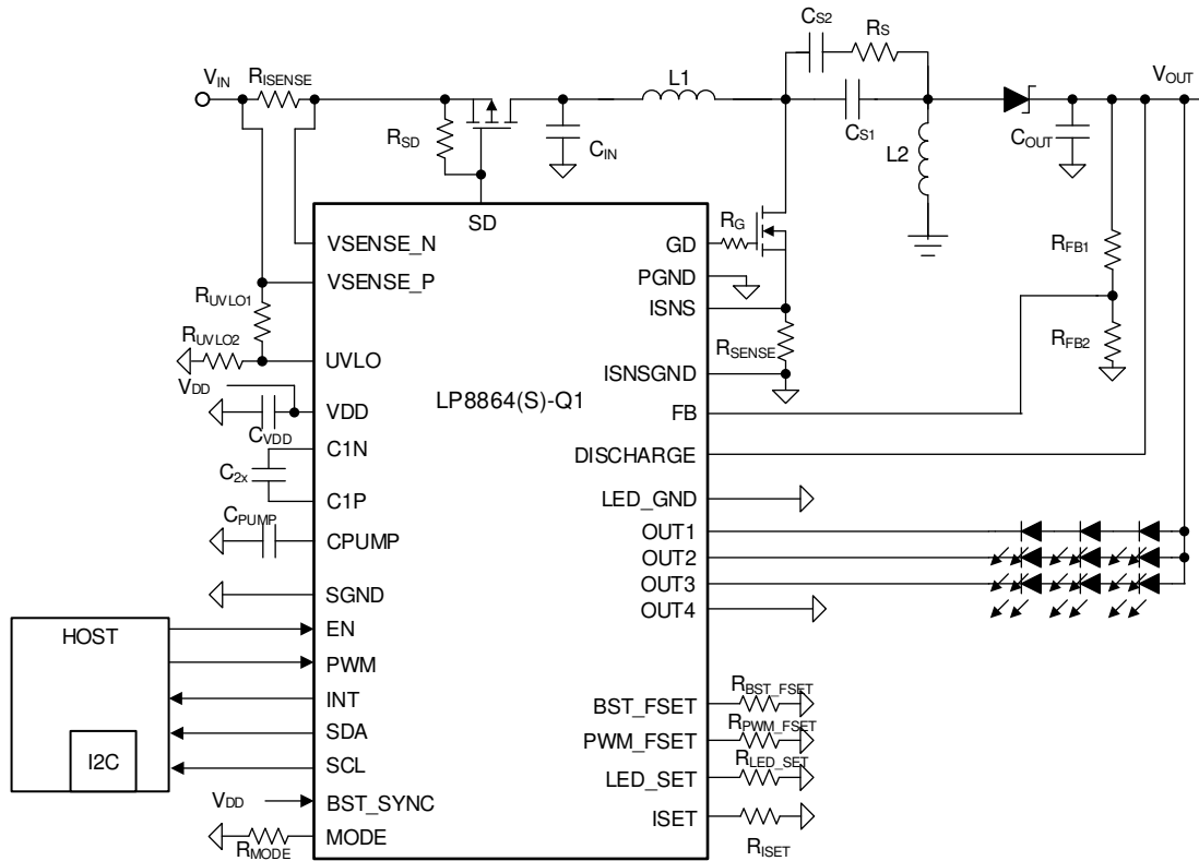
图 8-6. SEPIC Mode with Three LEDs in Series
