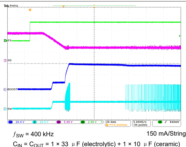
图 8-4. Typical Start-Up
