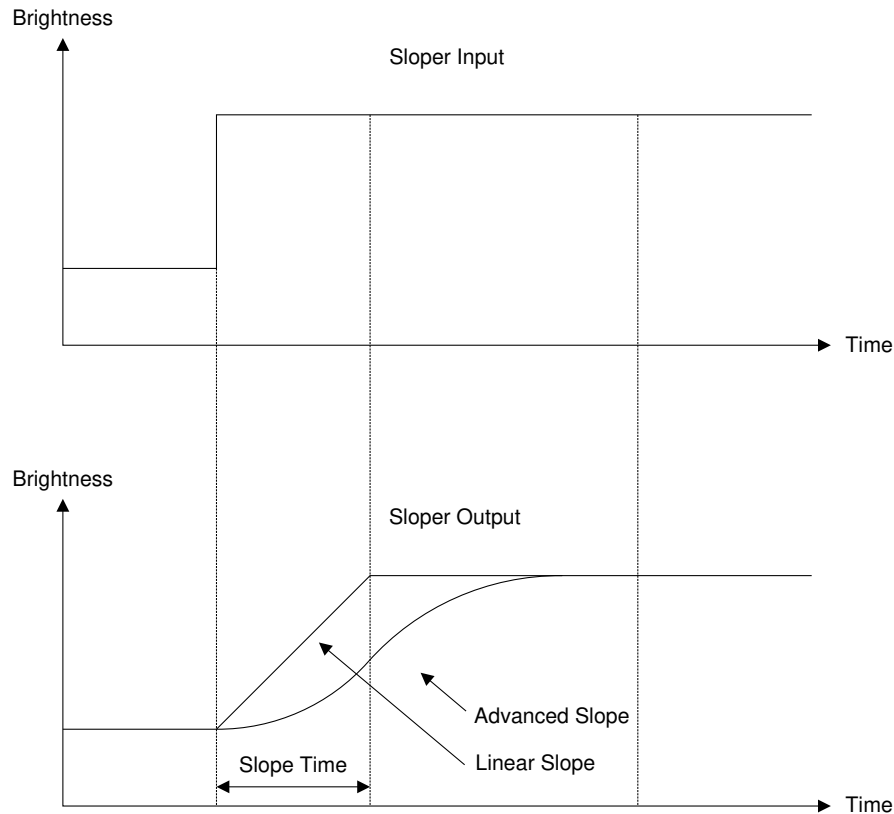
图 7-13. Brightness Sloper
