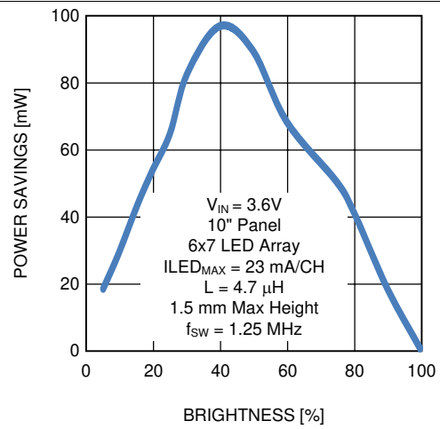
Figure 27. Power Savings With Adaptive Dimming when Compared to PWM Dimming
