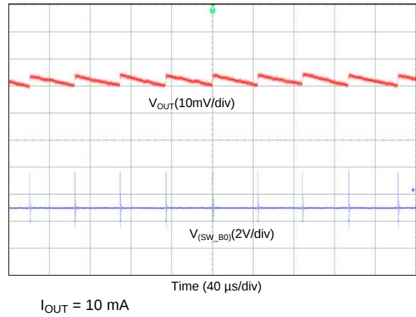
图 77. Output Voltage Ripple, PFM Mode (4-Phase Output)
