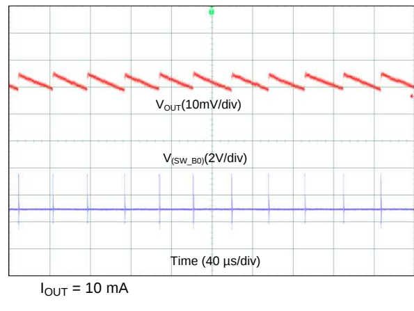
图 79. Output Voltage Ripple, PFM Mode (2-Phase Output)
