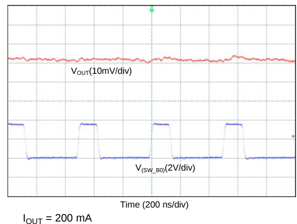
图 81. Output Voltage Ripple, Forced-PWM Mode (4-Phase Output)
