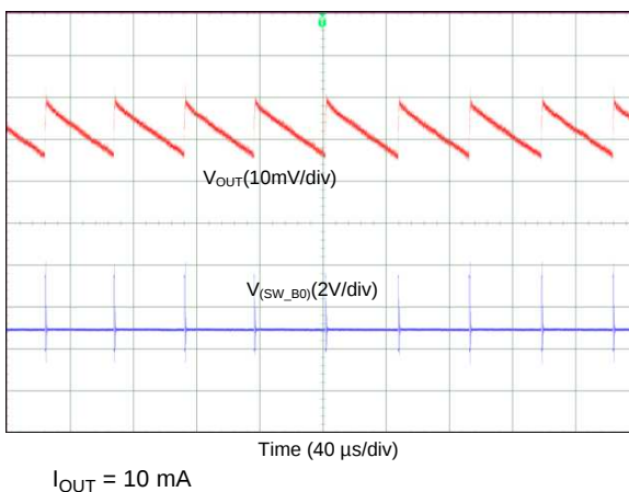
图 80. Output Voltage Ripple, PFM Mode (1-Phase Output)
