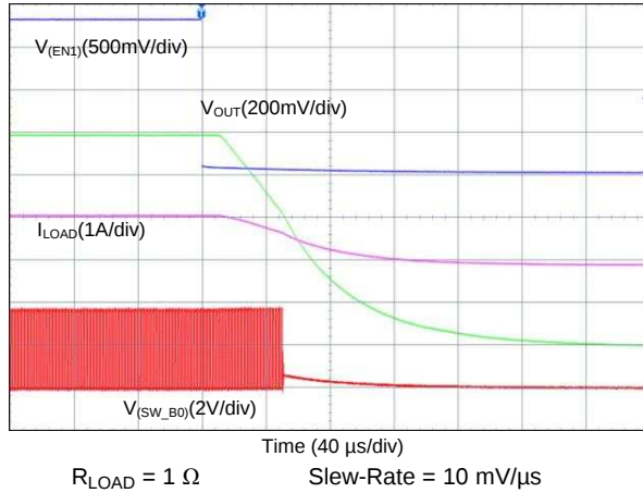
图 76. Shutdown With EN1, Forced PWM (1-Phase Output)
