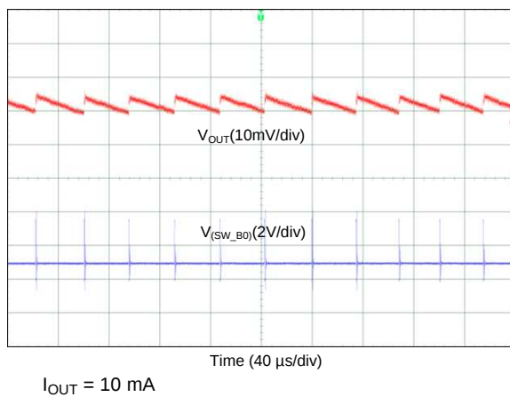
图 78. Output Voltage Ripple, PFM Mode (3-Phase Output)
