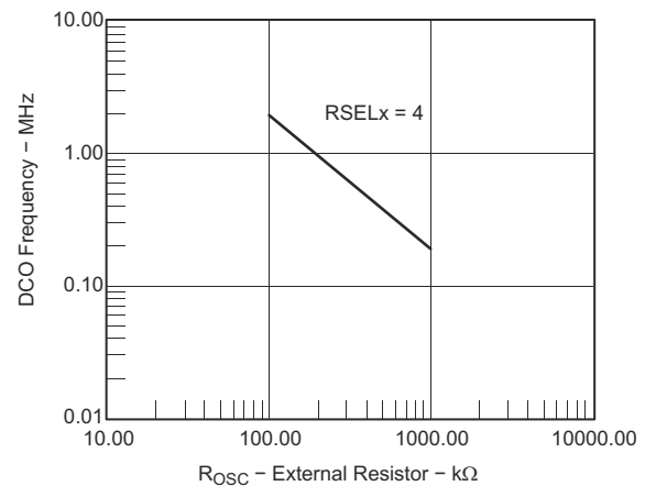
图 8-20. DCO Frequency vs R_{OSC} ( V_{CC} = 3\text{ V} , T_A = 25^\circ\text{C} )
