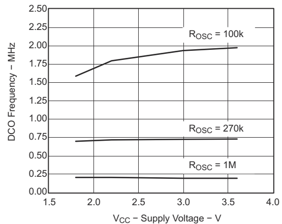
图 8-22. DCO Frequency vs Supply Voltage ( T_A = 25^\circ\text{C} )
