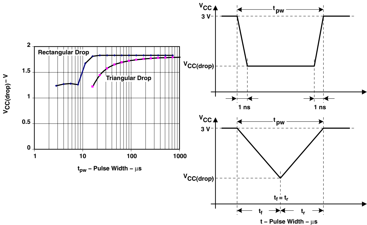
Figure 14. V_{CC(drop)} With a Square Voltage Drop and a Triangle Voltage Drop to Generate an SSVS Signal
