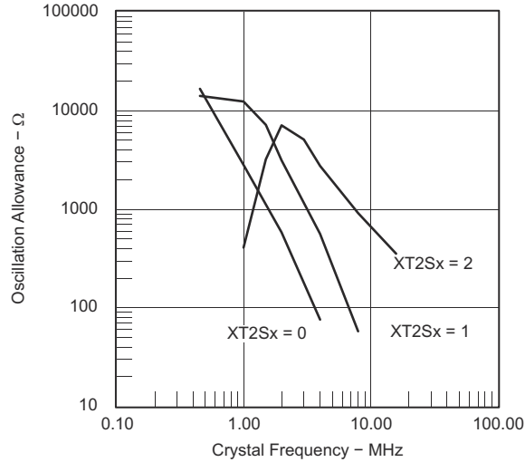
图 8-25. Oscillation Allowance vs Crystal Frequency C_{L,eff} = 15 \text{ pF} , T_A = 25^\circ\text{C}
