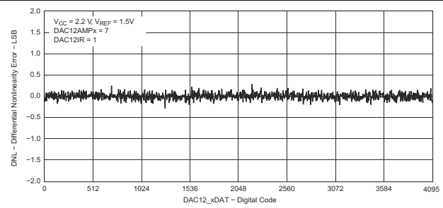
图 8-43. Typical DNL Error vs Digital Input Data
