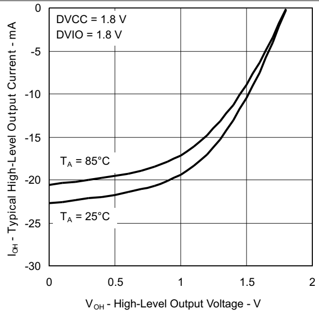
Figure 5-21. Typical High-Level Output Current vs High-Level Output Voltage
