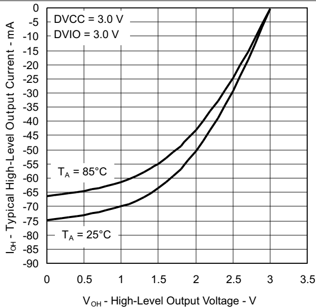
Figure 5-20. Typical High-Level Output Current vs High-Level Output Voltage
