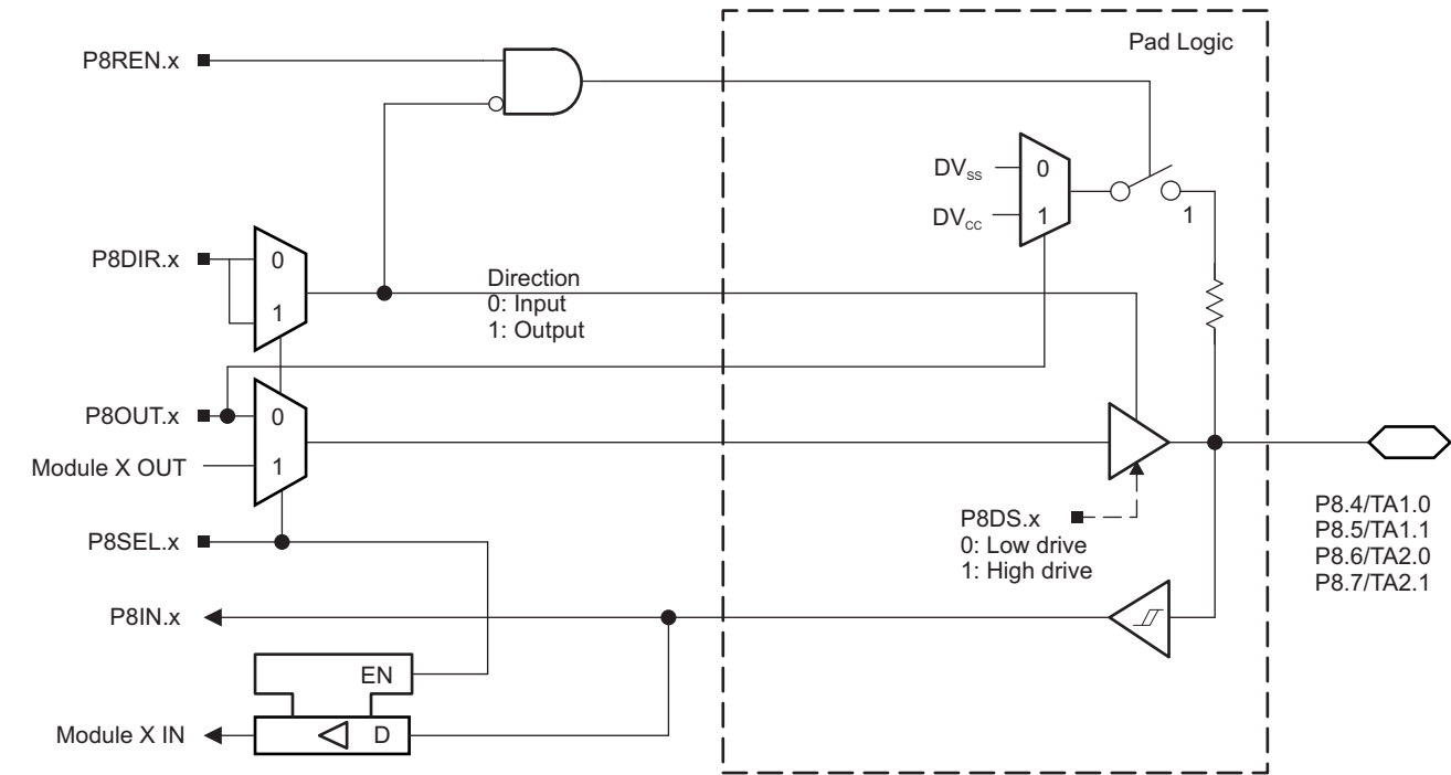
图 6-10. Port P8 (P8.4 to P8.7) Diagram (MSP430F67xxIPZ Only)
