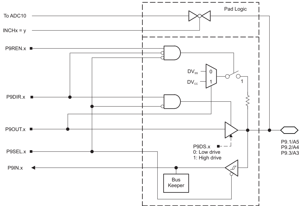
图 6-12. Port P9 (P9.1 to P9.3) Diagram (MSP430F67xxIPZ Only)
