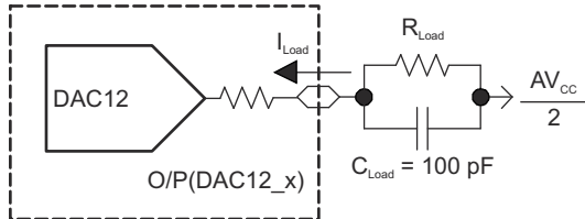
图 8-18. DAC12_x Output Resistance Tests
