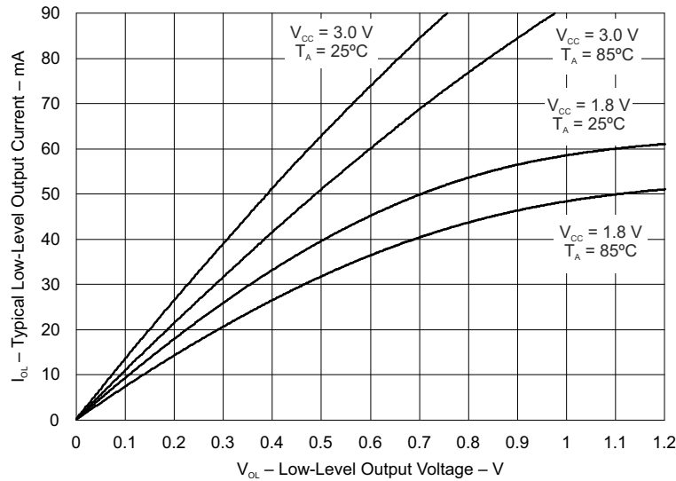
图 8-23. Ports PU.0, PU.1 Typical Low-Level Output Characteristics
