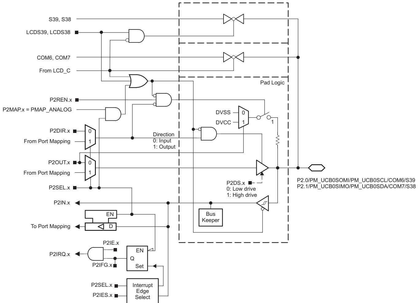
图 6-13. Port P2 (P2.0 and P2.1) Diagram (MSP430F67xxIPN Only)
