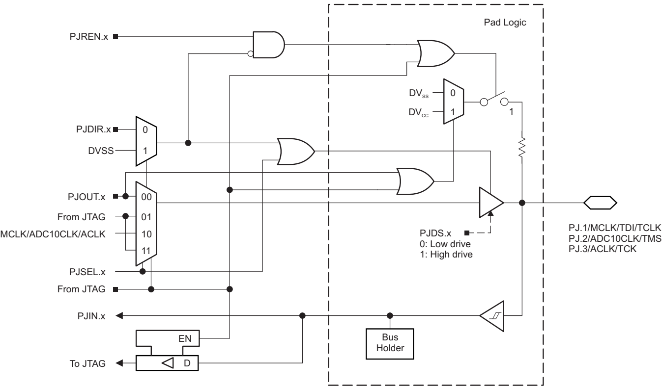
图 6-18. Port PJ (PJ.1 to PJ.3) Diagram
