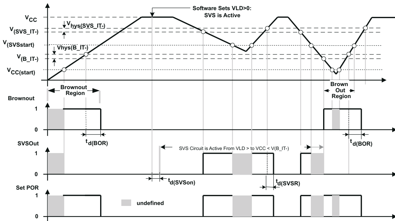
Figure 8-13. SVS Reset (SVSR) vs Supply Voltage
