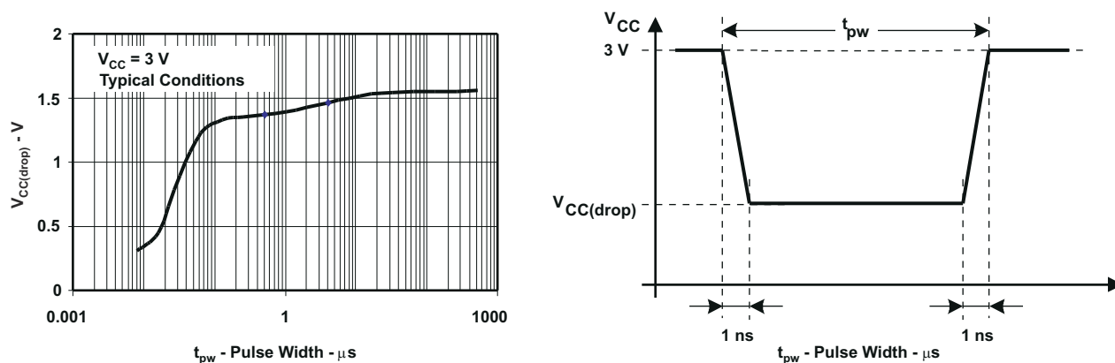
Figure 8-11. V_{CC(drop)} Level with a Square Voltage Drop to Generate a POR or BOR Signal
