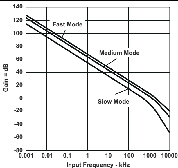
Figure 8-30. Typical Open-Loop Gain vs Frequency
