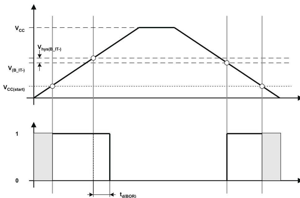
Figure 8-10. POR and BOR vs Supply Voltage
