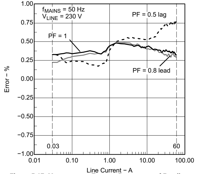
Figure 5-17. Measurement Error as Percentage of Reading (T A = –40°C)
