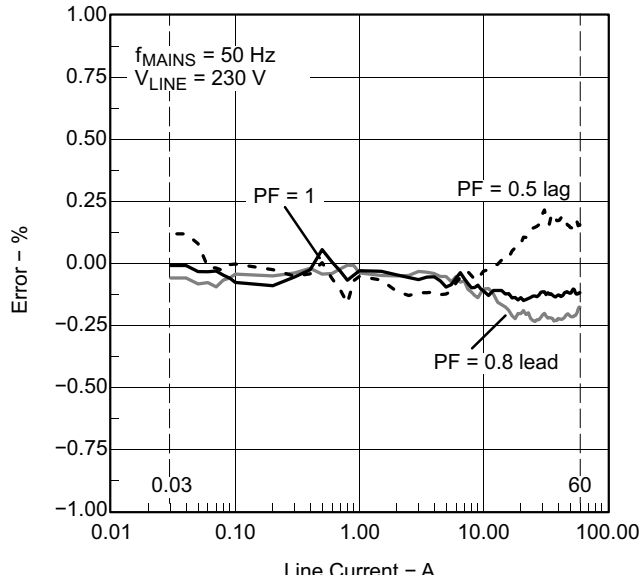
Figure 5-16. Measurement Error as Percentage of Reading (T A = 25°C)
