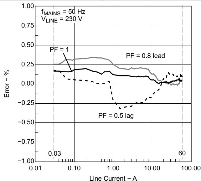
Figure 5-18. Measurement Error as Percentage of Reading (T A = 85°C)
