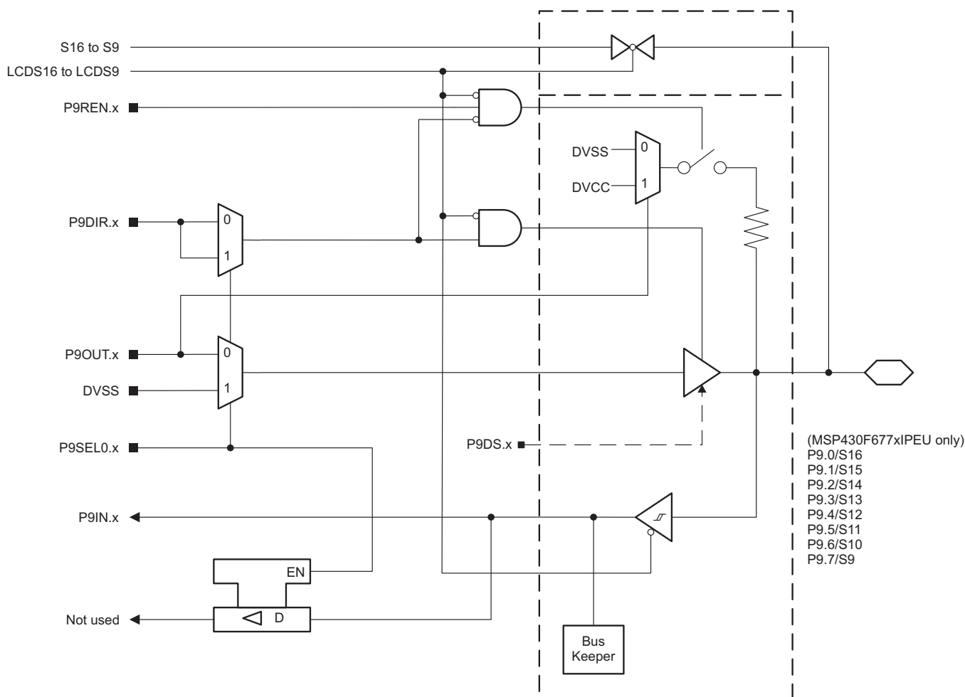
Figure 6-32. Port P9 (P9.0 to P9.7) Diagram (MSP430F677xIPEU Only)
