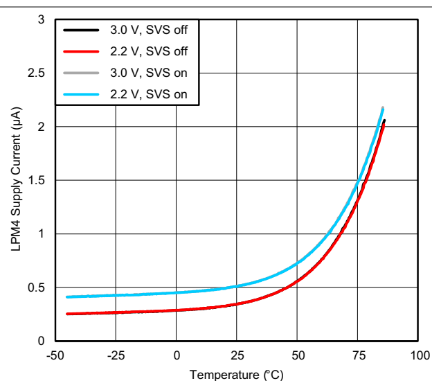
图 8-3. LPM4 Supply Current vs Temperature (LPM4,SVS)
