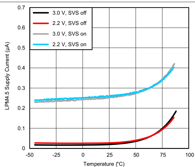
图 8-5. LPM4.5 Supply Current vs Temperature (LPM4.5)
