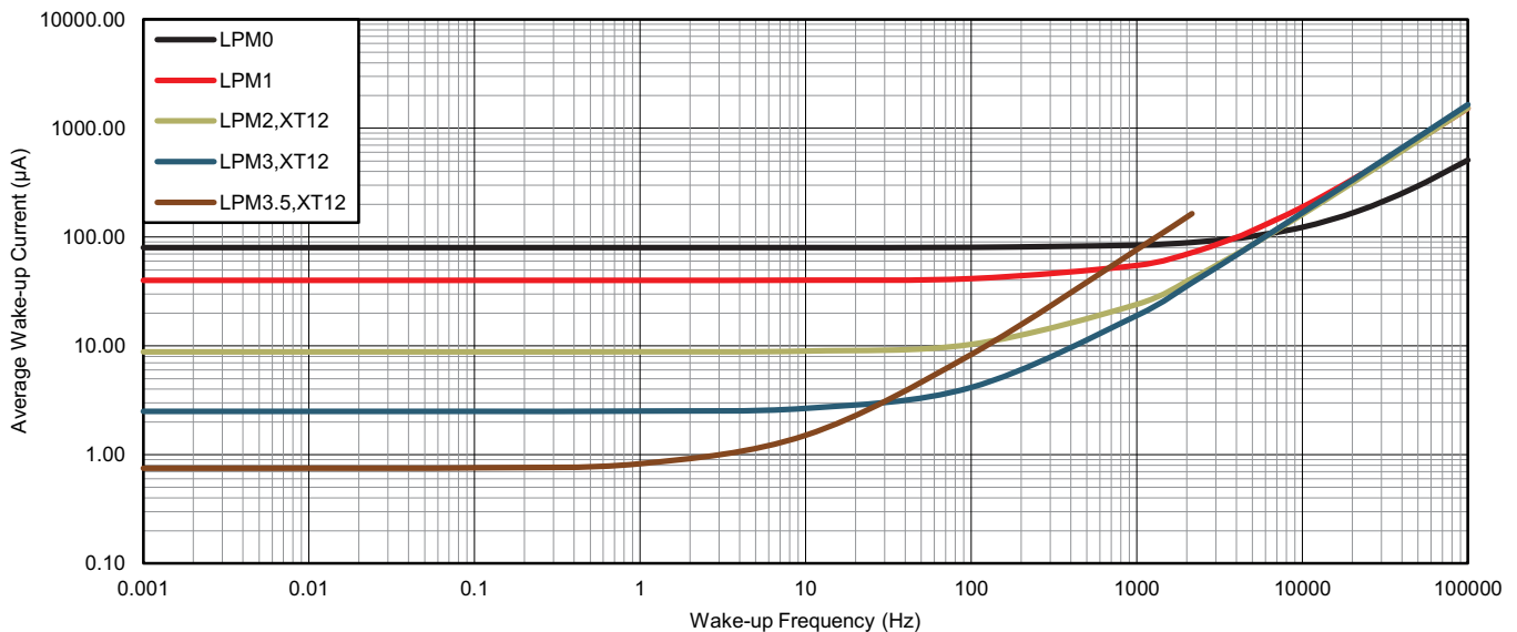
图 5-7. Average LPM Currents vs Wake-up Frequency at 85°C
