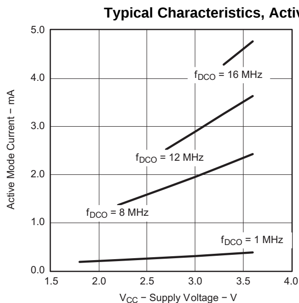
Figure 2. Active Mode Current vs V_{CC} , T_A = 25^\circ C
