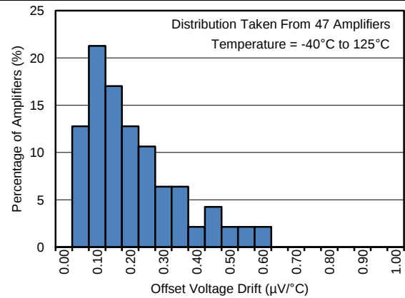
图 2. Offset Voltage Drift Production Distribution
