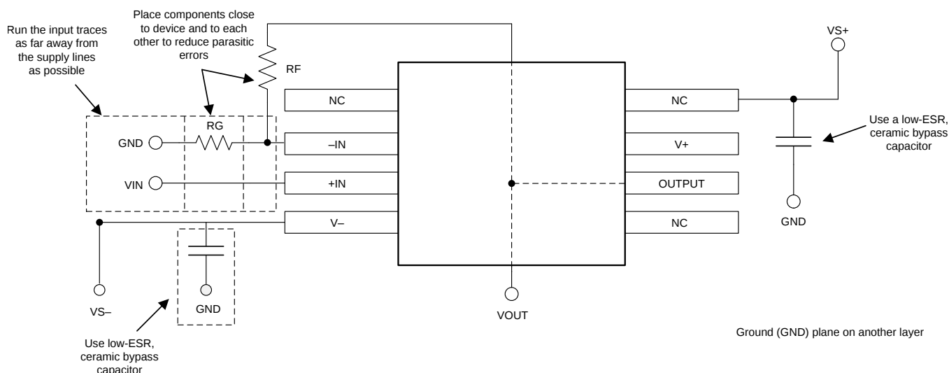
图 52. Operational Amplifier Board Layout for Noninverting Configuration
