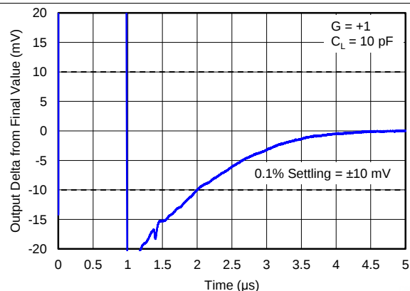
图 34. Large-Signal Step Response (10 V, G = +1 )
