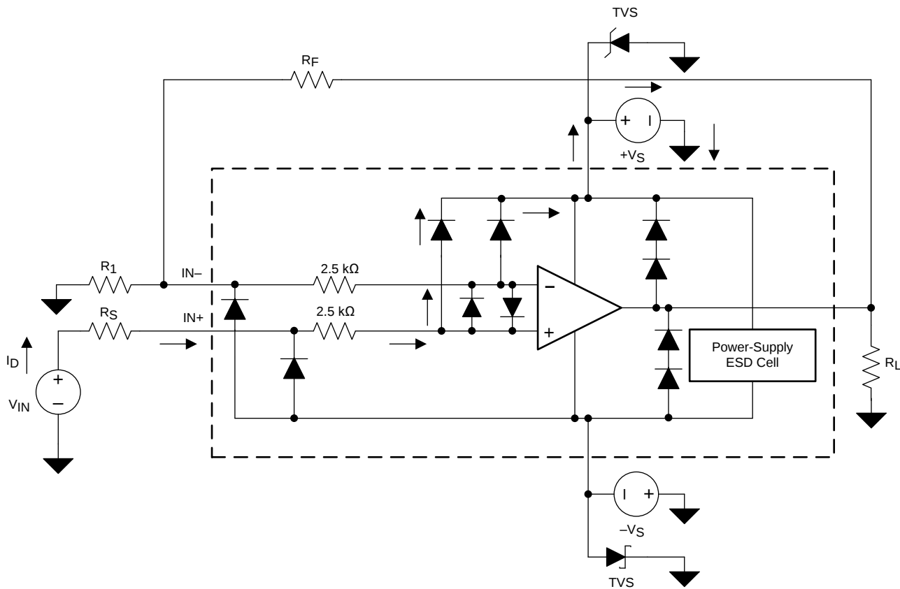
图 46. Equivalent Internal ESD Circuitry Relative to a Typical Circuit Application
