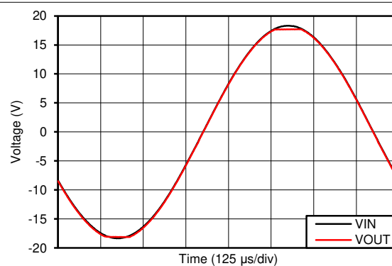
Figure 6-28. Positive Overload Recovery
