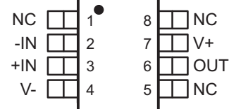
HKJ PACKAGE (TOP VIEW)
