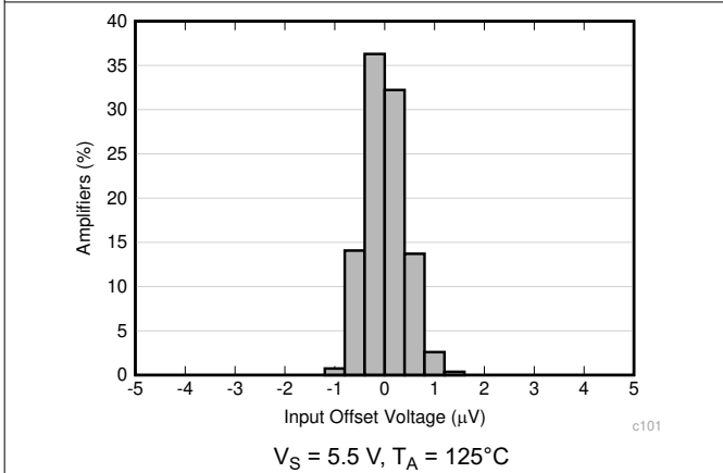
图 6-3. Offset Voltage Distribution
