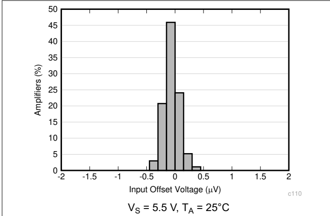
图 6-1. Offset Voltage Distribution
