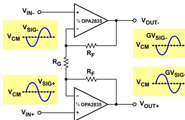
图 9-5. Differential-to-Differential Amplifier
