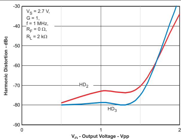
图 7-9. Harmonic Distortion vs Output Voltage
