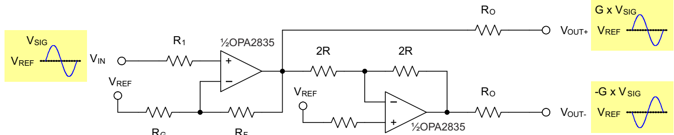
图 9-2. Single-Ended to Differential Amplifier
