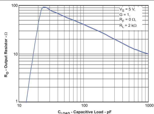
图 7-41. Series Output Resistor vs Capacitive Load
