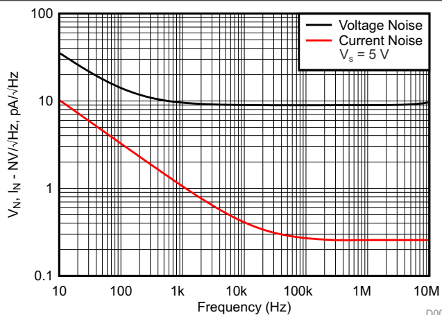
图 7-42. Input Referred Noise vs Frequency
