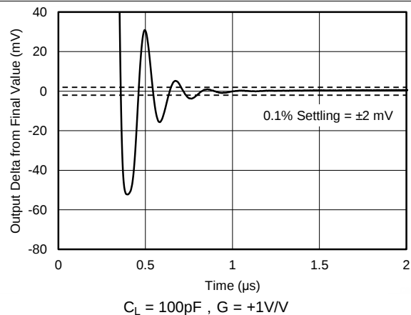
Figure 32. 负极性大信号趋稳时间
