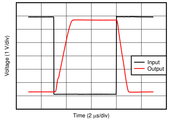
图 7-30. Overload Recovery
