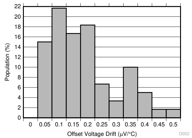
图 7-40. Offset Voltage Drift Distribution
