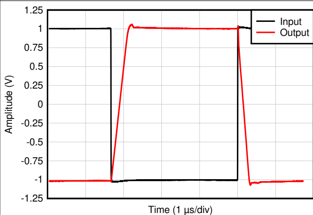
图 7-64. Small-Signal Step Response
