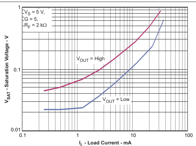
图 7-38. Output Saturation Voltage vs Load Current
