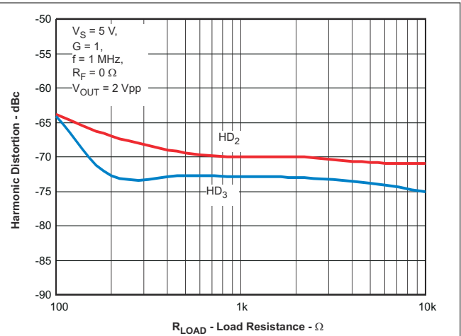
图 7-34. Harmonic Distortion vs Load Resistance
