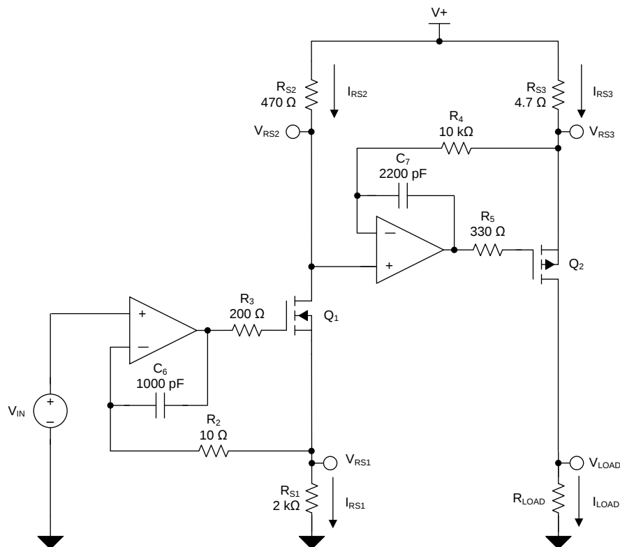
41. High-Side Voltage-to-Current (V-I) Converter
