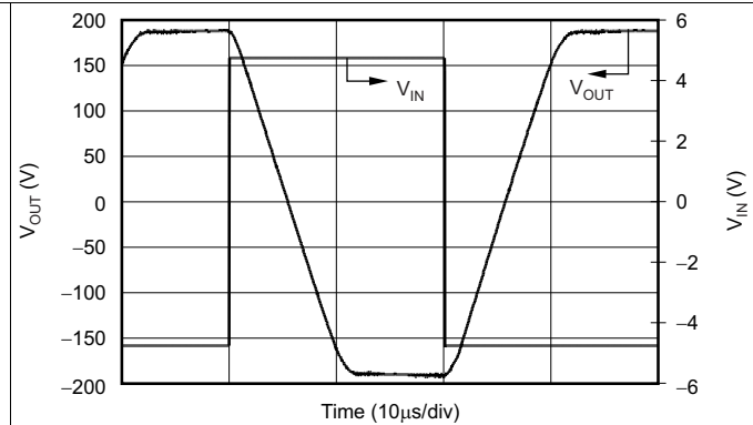
SR of 34 V/ms, which is significantly higher than the specified 13 V/ms due to tracking of the power-supply voltage Figure 83. 7.5-kΩ Load, G = +20, Six OPA454s, 100-V Supplies
