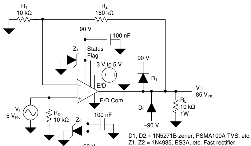
图 61. OPA462, High-Voltage Noninverting Amplifier, A_V = 17 V/V
