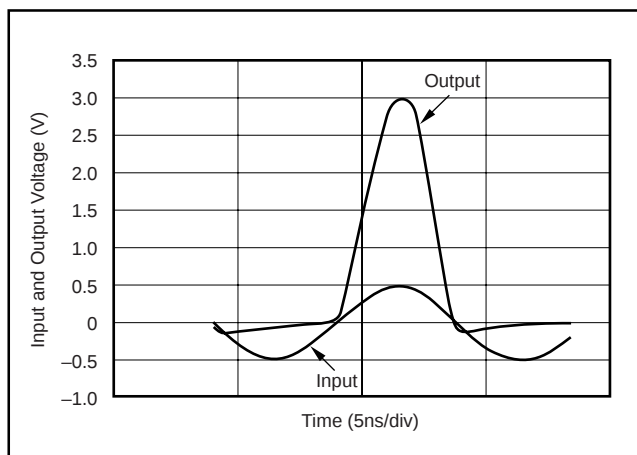
FIGURE 9. 100MHz Sinewave Rectified.
