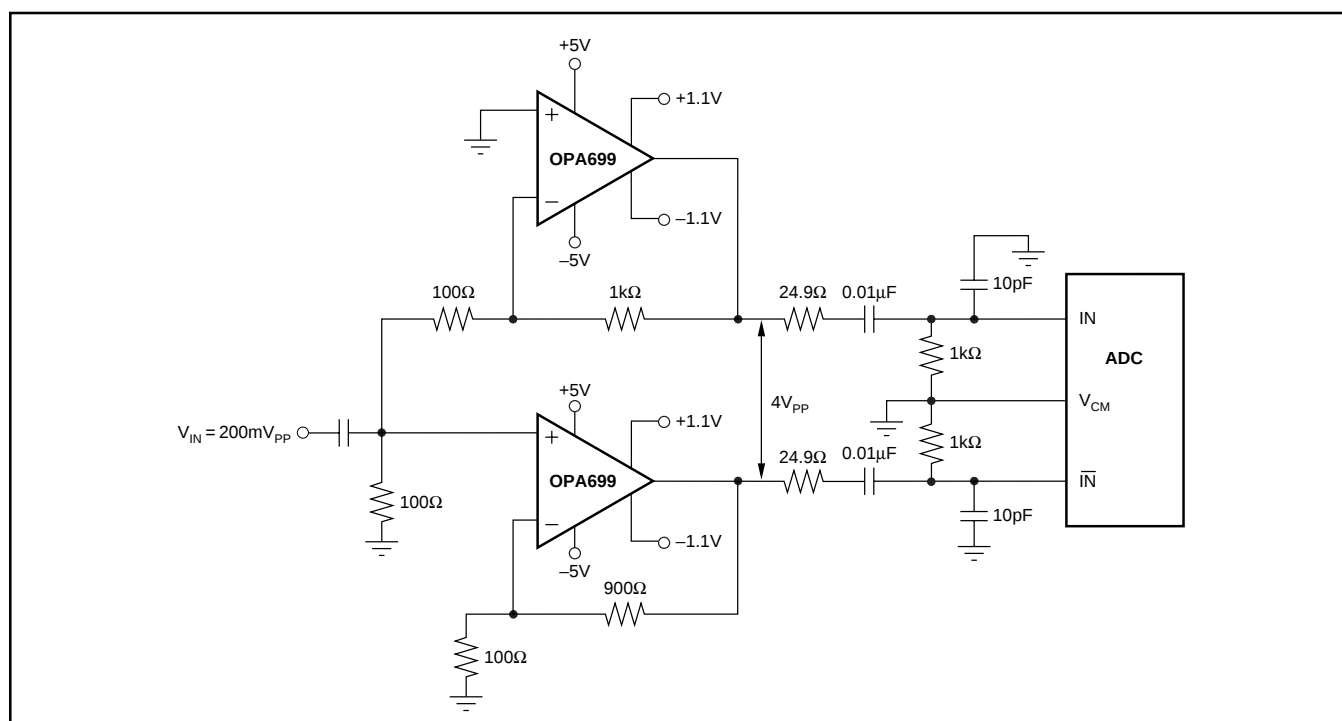
FIGURE 7. Single to Differential AC-Coupled, High Gain Output Limited ADC Driver.
