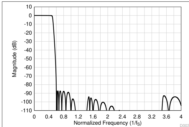
图 8-49. Ultra-Low-Latency Decimation Filter Magnitude Response
