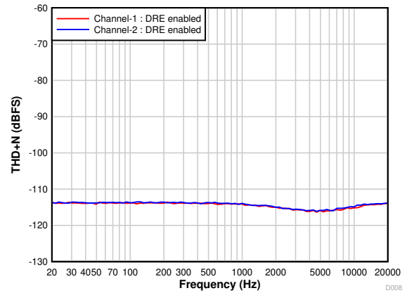
图 7-11. THD+N vs Input Frequency at -60-dBr Input With DRE Disabled
