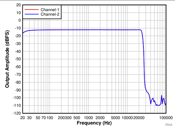
图 7-15. Frequency Response With a -12-dBr Input
