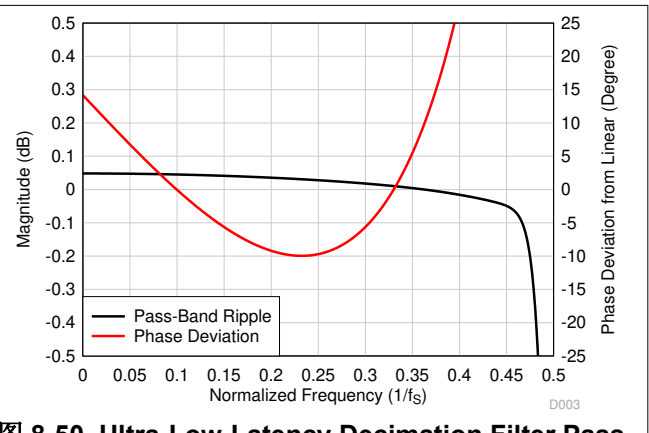
图 8-50. Ultra-Low-Latency Decimation Filter Pass-Band Ripple and Phase Deviation
