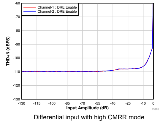
图 7-29. THD+N vs Input Amplitude With DRE Enabled
