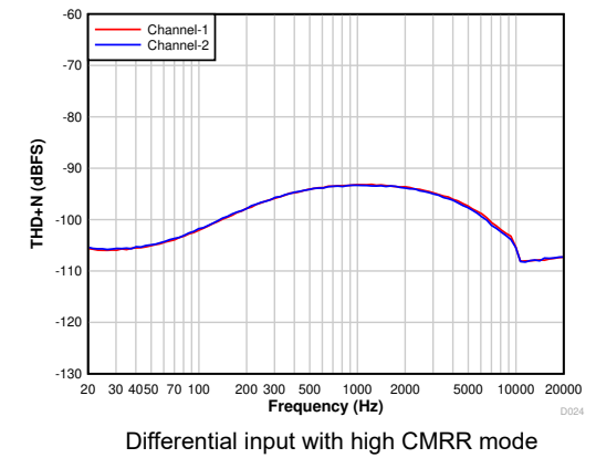
图 7-31. THD+N vs Input Frequency at -1-dBr Input With DRE Disabled
