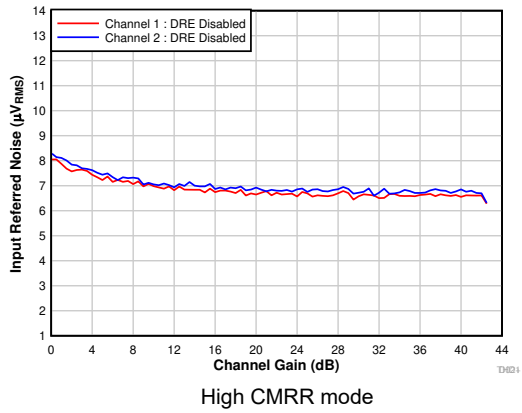
图 7-28. Input-Referred Noise vs Channel Gain
