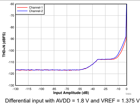
图 7-8. THD+N vs Input Amplitude With DRE Enabled
