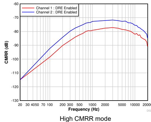
图 7-27. Common-Mode Rejection Ratio vs Ripple Frequency With 100-mV pp Amplitude and DRE Enabled
