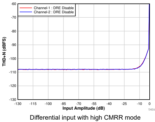
图 7-30. THD+N vs Input Amplitude With DRE Disabled
