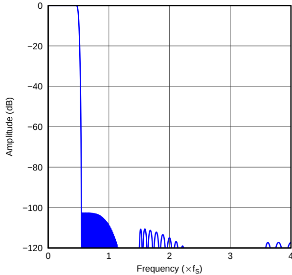
Figure 49. High-Attenuation x8 Interpolation Filter Frequency Response, Single Rate
