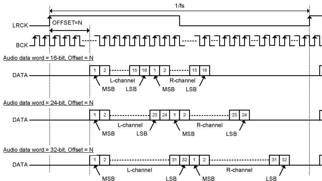
Figure 21. TDM/DSP 3 Audio Data Format
