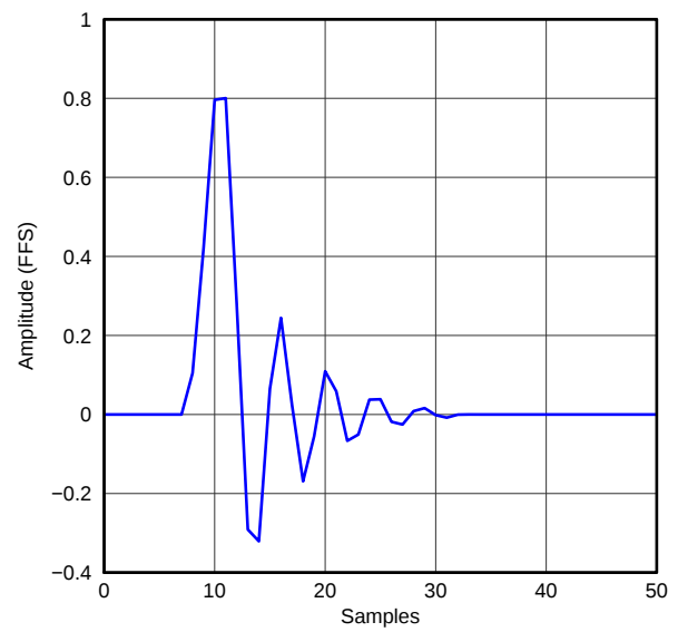
Figure 47. Asymmetric FIR x2 Interpolation Filter Impulse Response, Quad Rate
