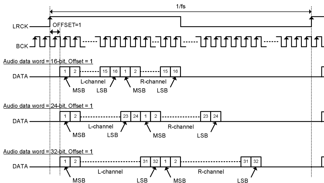
Figure 20. TDM/DSP 2 Audio Data Format
