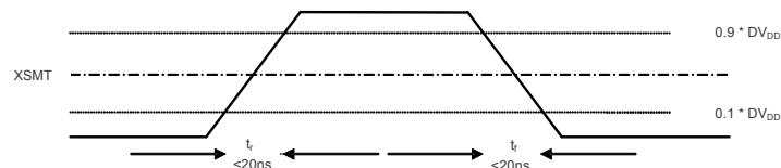
Figure 7. XSMT Timing for Soft Mute and Soft Un-Mute
