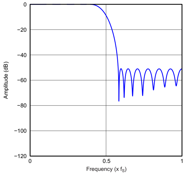
Figure 46. Asymmetric FIR x2 Interpolation Filter Frequency Response, Quad Rate
