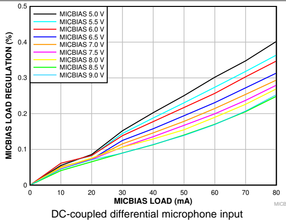
图 18. MICBIAS Load Regulation vs MICBIAS Load Current
