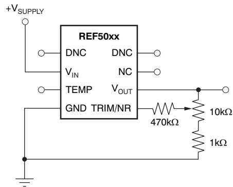
Figure 41. V OUT Adjustment Using the TRIM/NR Pin
