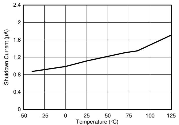
图 7-12. Shutdown Current vs Temperature
