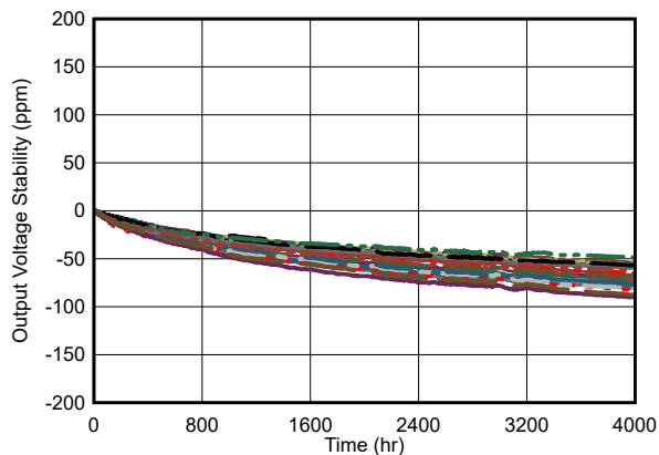
图 7-20. Long-Term Stability (First 4000 Hours)
