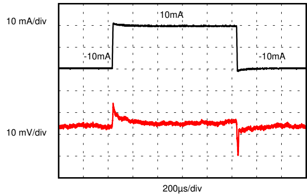
图 7-8. Load Transient Response ( C_L = 1\text{ }\mu\text{F} )
