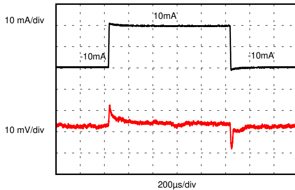
图 7-9. Load Transient Response ( C_L = 10\text{ }\mu\text{F} )
