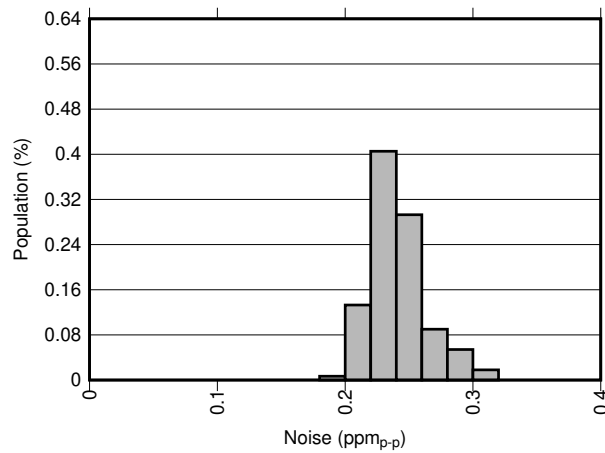
图 7-15. 0.1-Hz to 10-Hz Voltage Noise Distribution (300 units)
