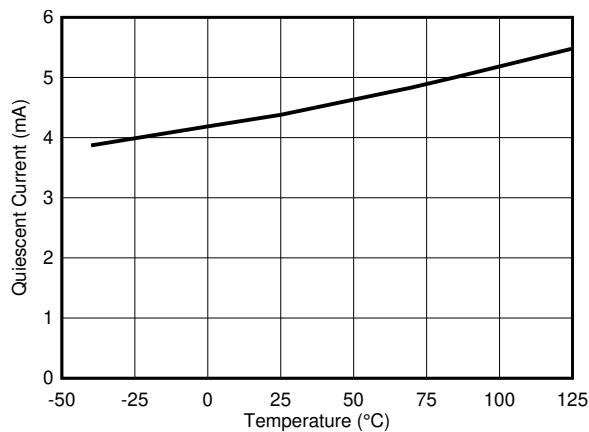
图 7-11. Quiescent Current vs Temperature
