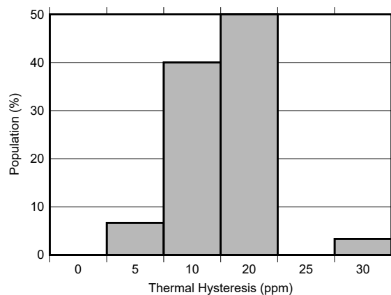
图 7-19. REF7012 FKH Thermal Hysteresis Distribution (0°C to 70°C)
