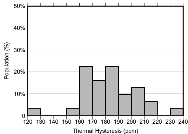
图 8-4. REF7025 Thermal Hysteresis Distribution (-40°C to 125°C)
