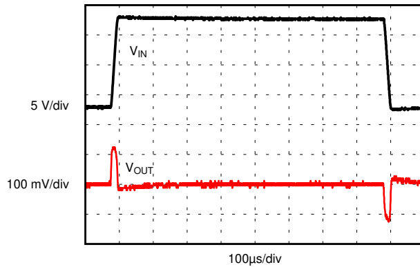
图 7-7. Line Regulation Response
