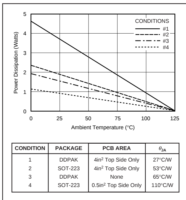
FIGURE 9. Maximum Power Dissipation versus Ambient Temperature for the Various Packages and PCB Heat Sink Configurations.
