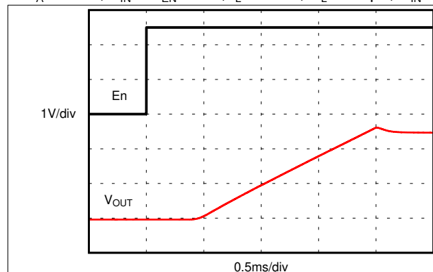
Figure 19. Turnon Time (Enable)
