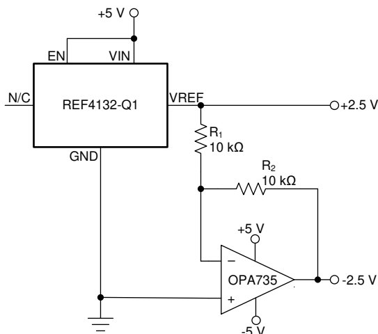
Simplified Schematic
