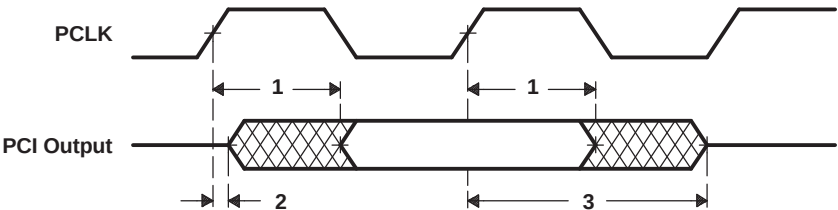
Figure 5-49. PCI Output Timing (33/66 MHz)
