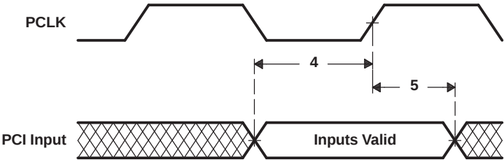
Figure 5-48. PCI Input Timing (33/66 MHz)
