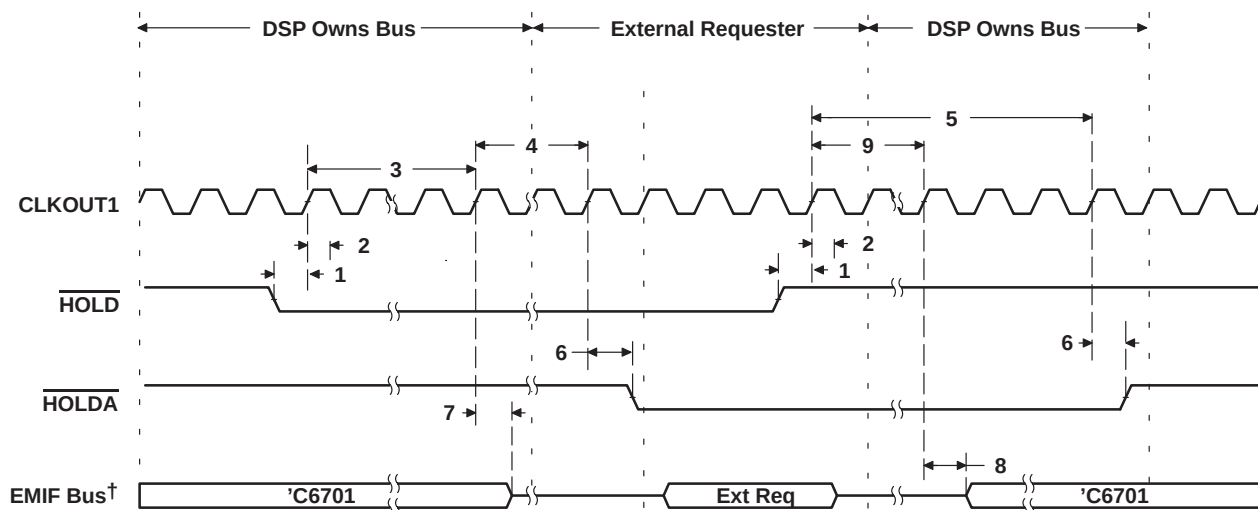
Figure 24. HOLD/HOLDA Timing
