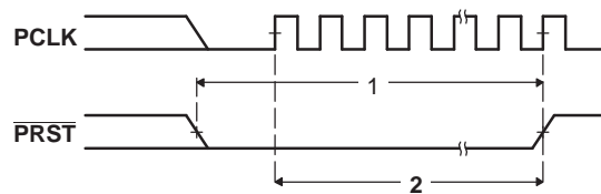
Figure 5-37. PCI Reset ( \overline{\text{PRST}} ) Timing
