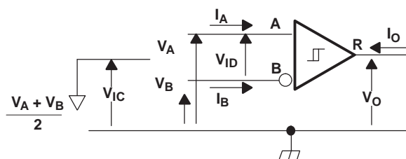
Figure 16. Receiver Voltage and Current Definitions
