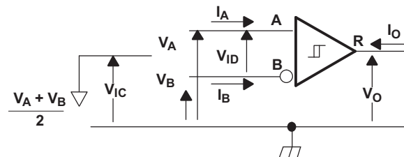
Figure 14. Receiver DC Parameter Definitions
