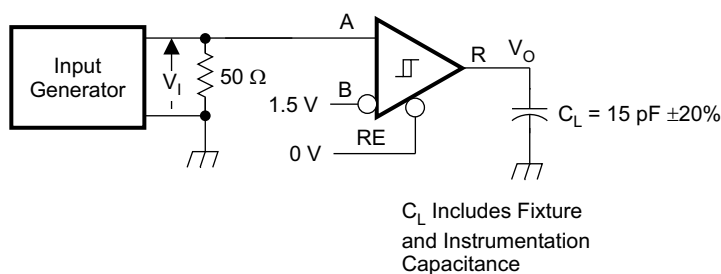
图 20. Measurement of Receiver Output Rise and Fall Times and Propagation Delays
