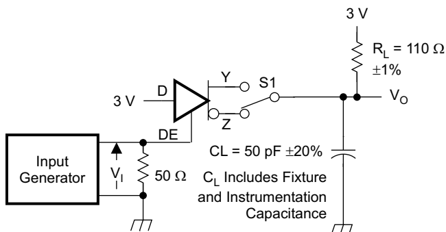
图 18. Measurement of Driver Enable and Disable Times with Active-High Output and Pulldown Load
