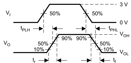
图 20. Measurement of Receiver Output Rise and Fall Times and Propagation Delays
