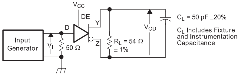
图 17. Measurement of Driver Differential Output Rise and Fall Times and Propagation Delays
