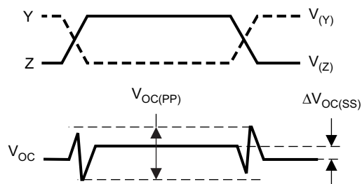
图 16. Measurement of Driver Differential and Common-Mode Output With RS-485 Load
