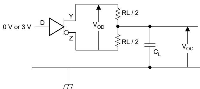
图 16. Measurement of Driver Differential and Common-Mode Output With RS-485 Load
