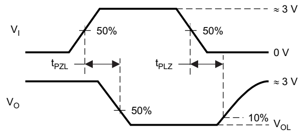
图 19. Measurement of Driver Enable and Disable Times with Active-Low Output and Pullup Load
