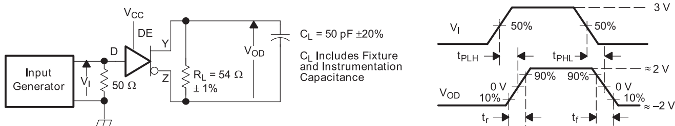
图 17. Measurement of Driver Differential Output Rise and Fall Times and Propagation Delays
