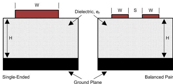
Figure 42. Microstrip Topology
