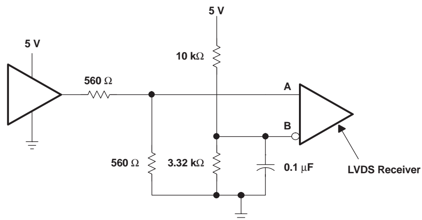
Figure 34. 5-V CMOS
