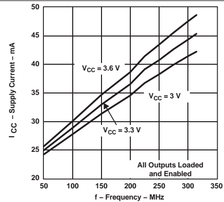
Figure 2. SN65LVDS105 Supply Current vs Frequency
