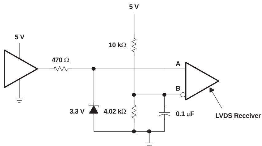
Figure 35. 5-V TTL
