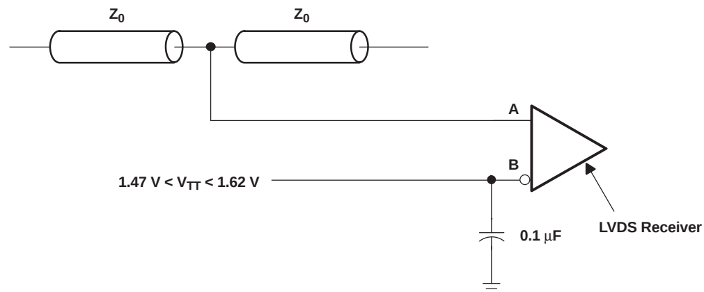
Figure 30. Backplane Transceiver
