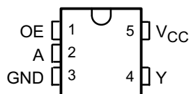
Pin Functions
