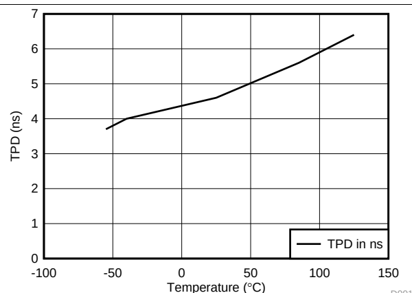
Figure 1. SN74AHCT245 TPD vs Temperature, 15 pF Load
