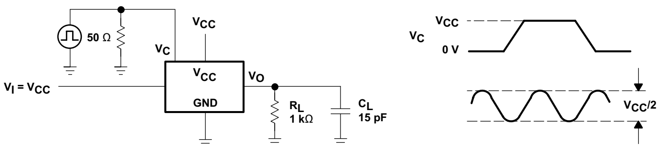
Figure 7. Control-Input Frequency
