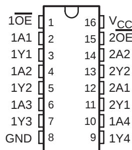
SN54LV367A . . . J OR W PACKAGE SN74LV367A . . . D, DB, DGV, NS, OR PW PACKAGE (TOP VIEW)
